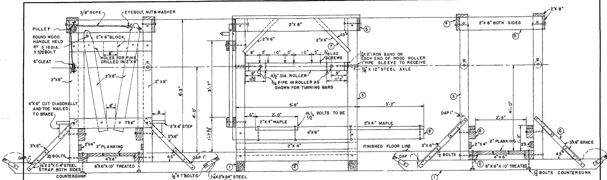
SIDE ELEVATION
