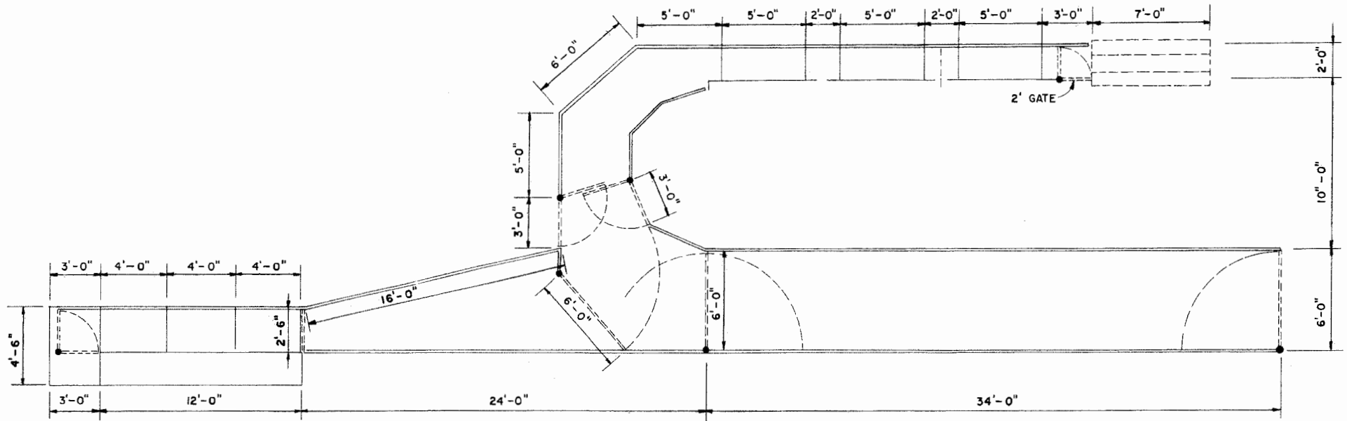
PLAN SCALE: 1/4" = 1'-0" 12' 0" 1' 2' 3' 4'
