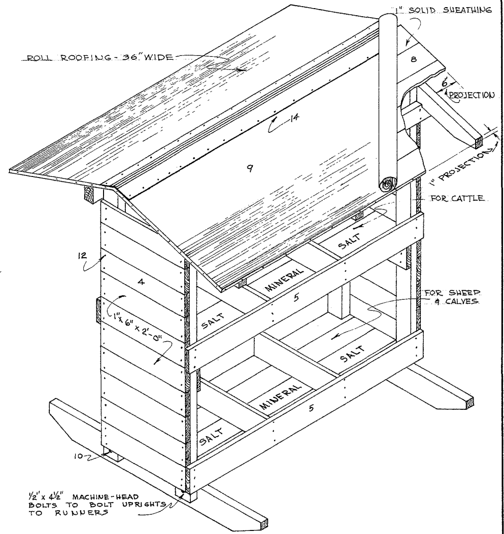
VIEW OF COMPLETE BOX
