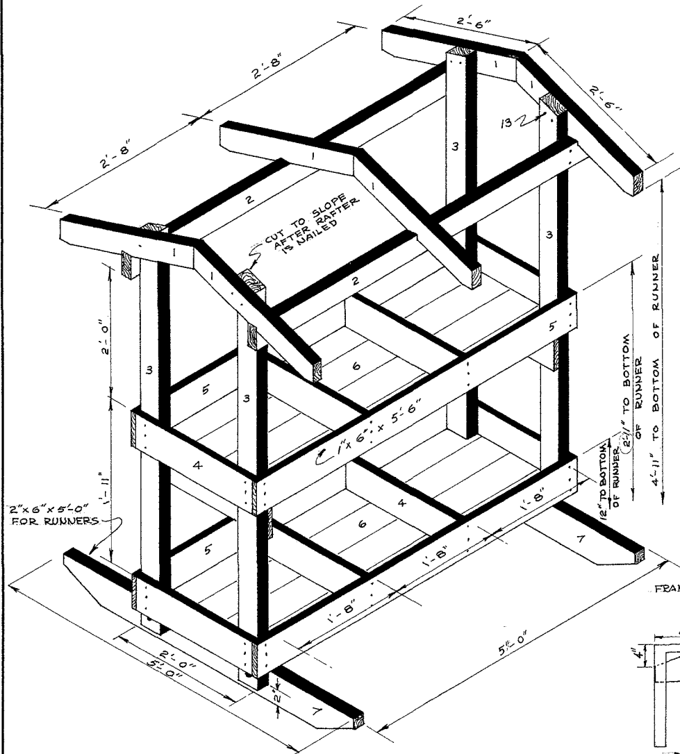
DETAILS OF FRAMING
