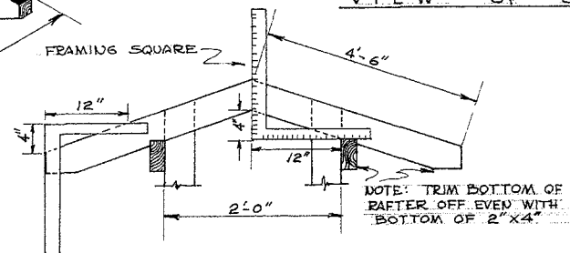
DETAILS OF RAFTER
