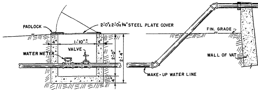
SECTION THRU VALVE BOX SCALE: 3/4" = 1'-0"
