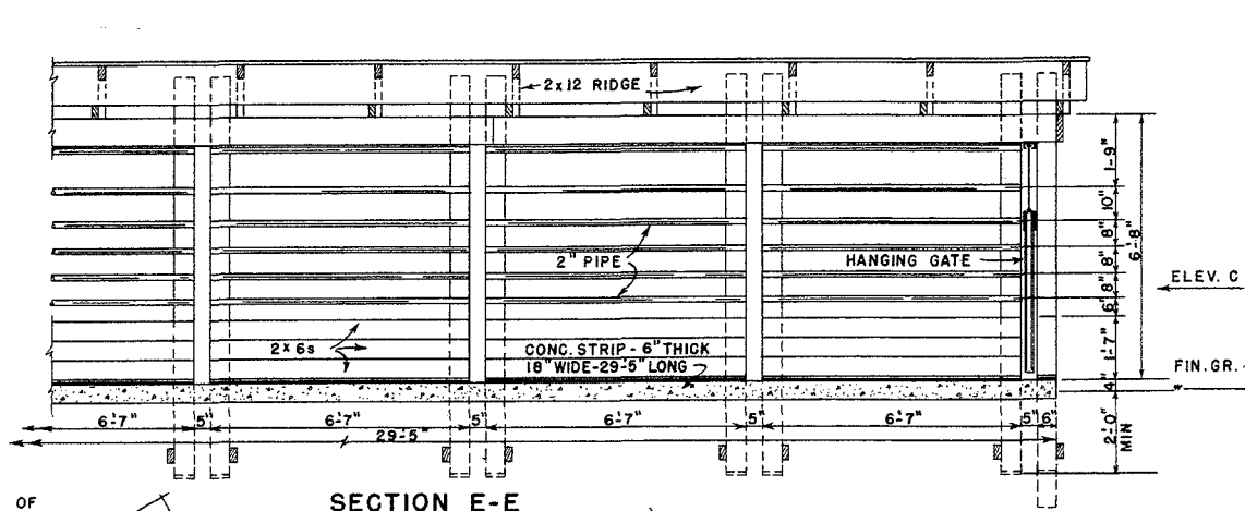
SECTION E-E
