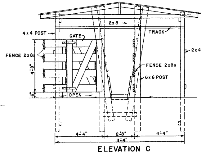
ELEVATION C
