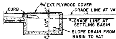
DETAIL "Y"
