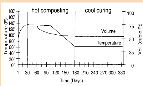
Figure 3. Temperature and volume changes in a static compost pile made with stall cleanings from horses bedded on wood shavings (Hamilton, 2002).
