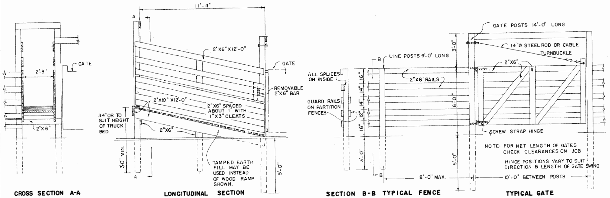
LOADING RAMP
