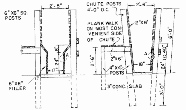
ALTERNATE CHUTE
